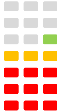
C [Fair] 65 – 74.99
