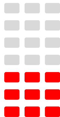
F [Fail] < 50
