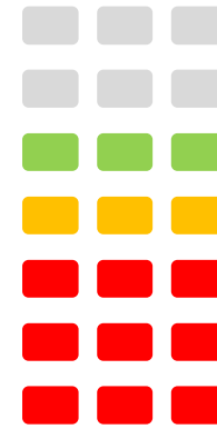
B [Good] 75 – 84.99
