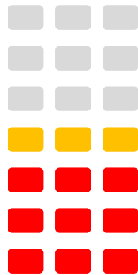
D [Poor] 55 – 64.99
